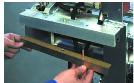
Top sideshift bearings are alloy bronze with grease nipples
